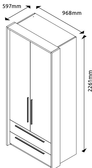
P22A/PN LWH - 968x597x2261
