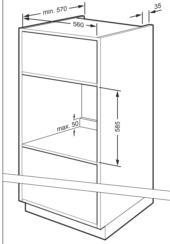
Installation in an upright cabinet
