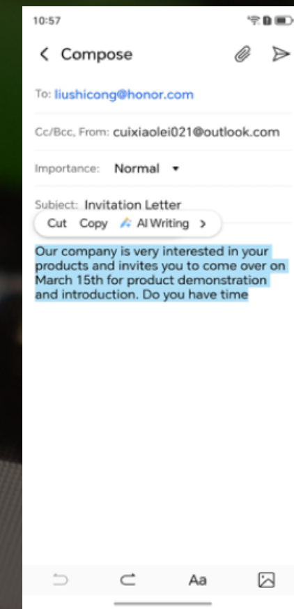
AI Creation
