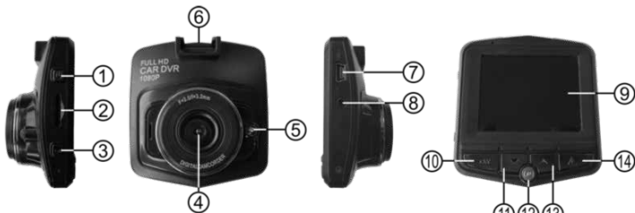
Figure 1: Camera
