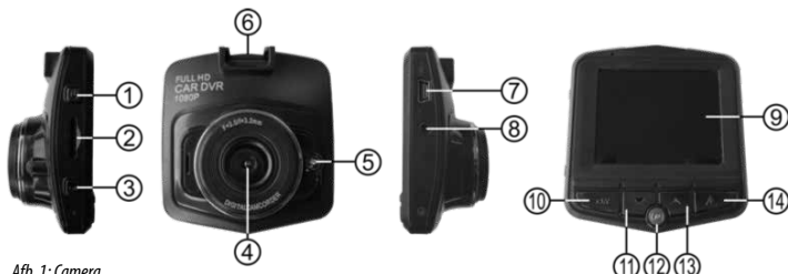
Afb. 1: Camera
