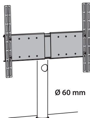
Universal VESA Adapter 100x100 - 600x400
