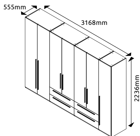
P74/PN LWH - 3168x0555x2236
