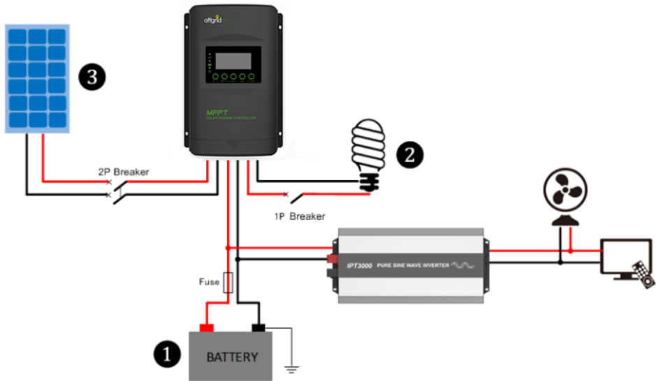
Figure 2.2 Schematic of wiring diagram
