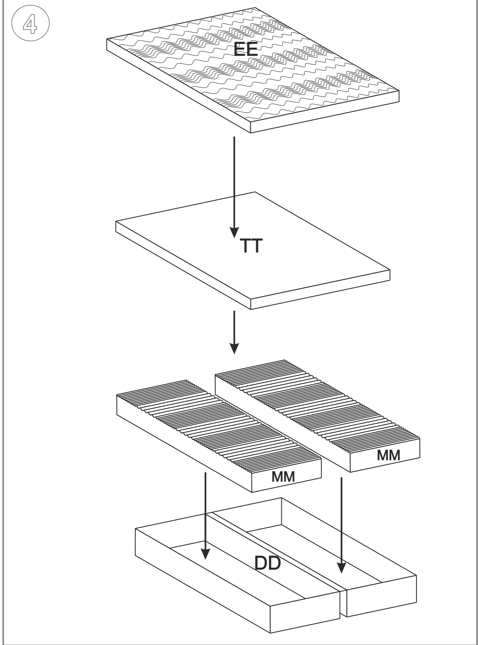
AMALFI 180 LED
