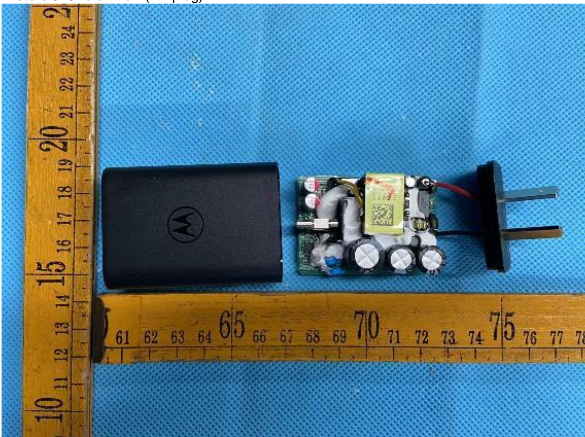
Picture 6. Internal view (AR plug)
