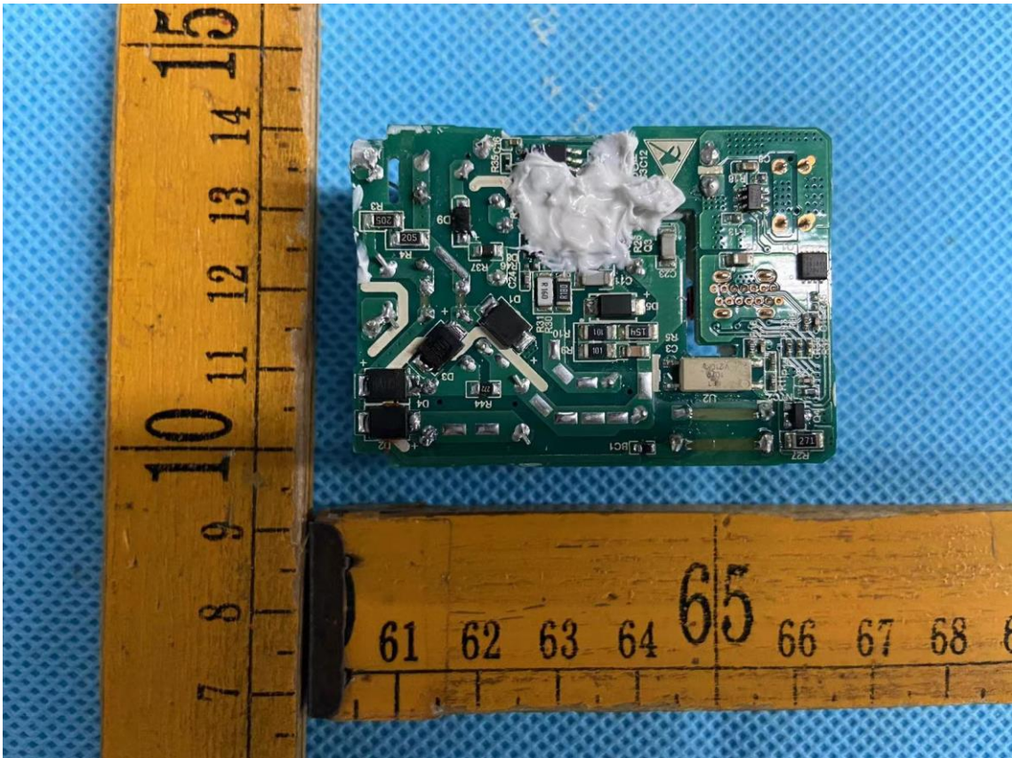
Picture 23.PCB trace view (final with glue)
