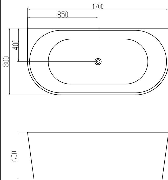
Horizontal dimensions
