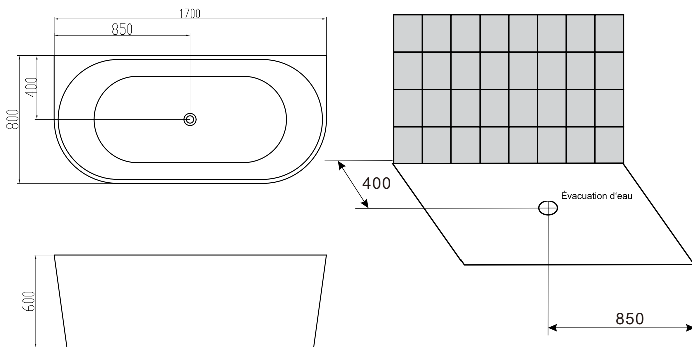
Dimensions section transversale
