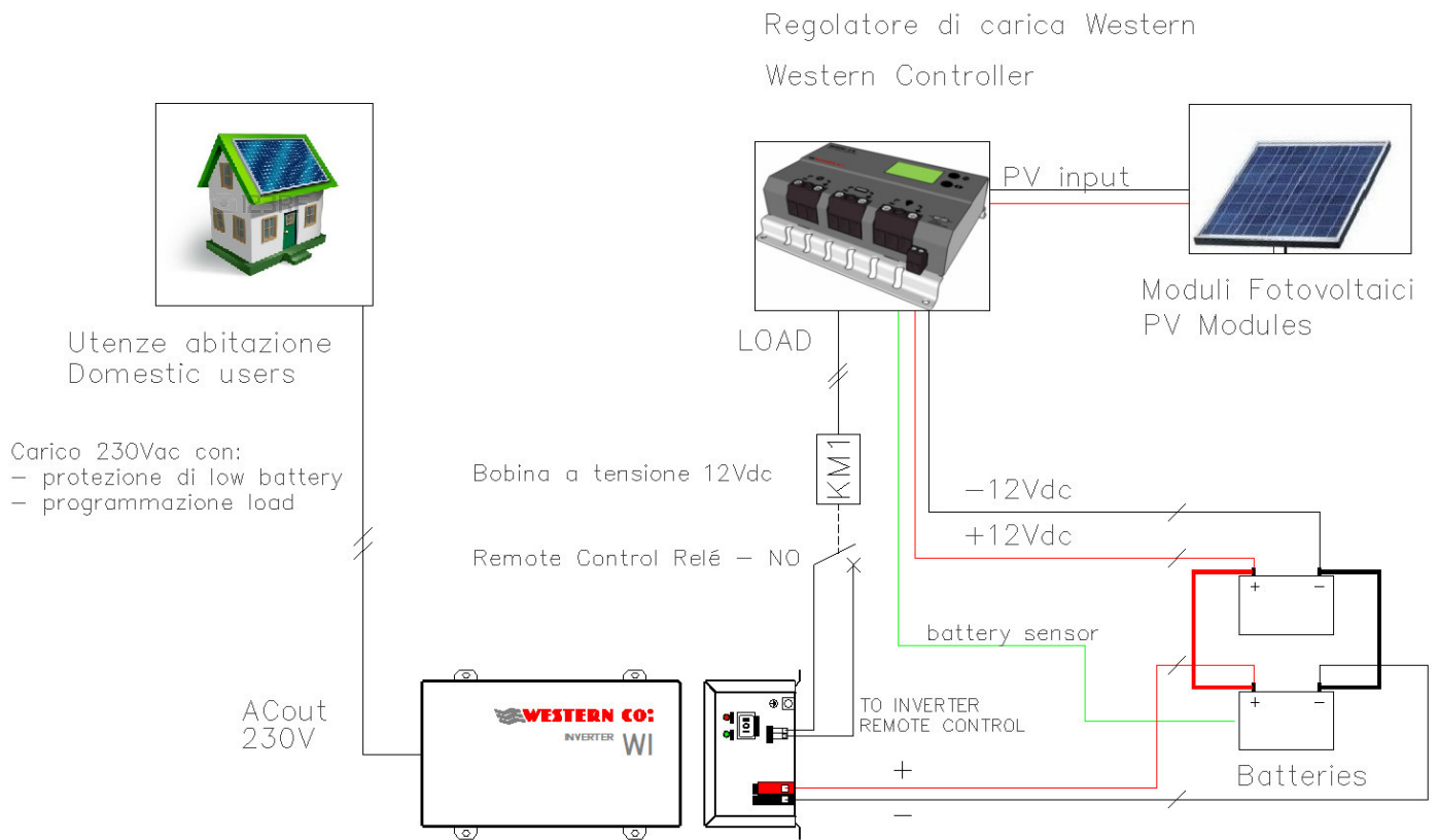
Pic. 3 WI800-12 Wiring scheme
